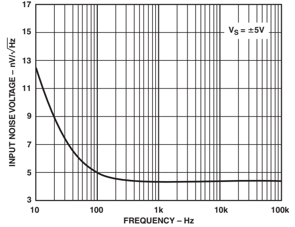
TPC 40. AD9632 Noise vs. Frequency
