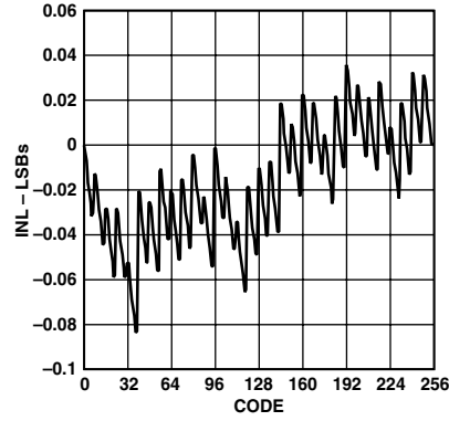
Figure 13. Typical INL
