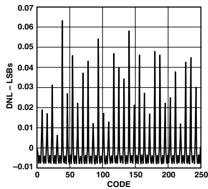
Figure 14. Typical DNL
