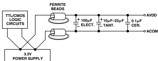
Figure 16. Differential LC Filter for Single 3.3 V Applications
