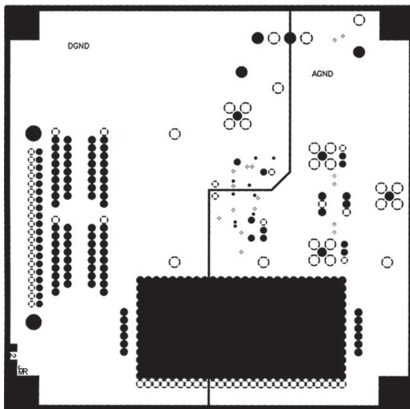
Figure 21. Ground Plane
