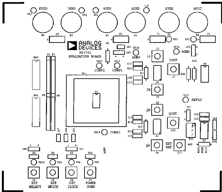
Figure 43. Silkscreen Layer—Top
