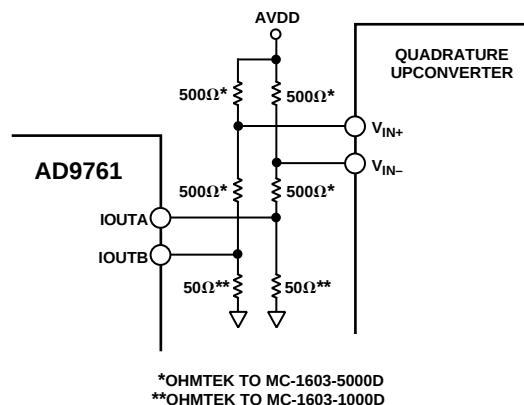
Figure 39. Differential, DC Coupled Output Configuration with Level-Shifting
