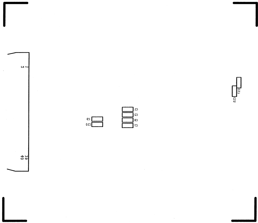
Figure 48. Silkscreen Layer—Bottom
