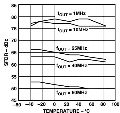
Figure 15. SFDR vs. Temperature @ 125 MSPS, 0 dBFS
