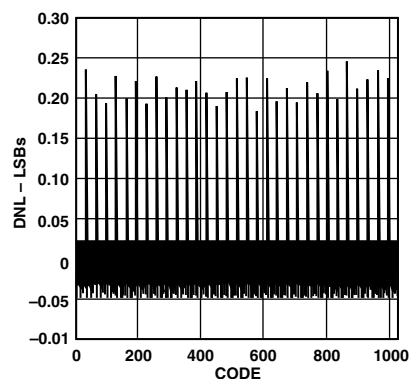
Figure 14. Typical DNL
