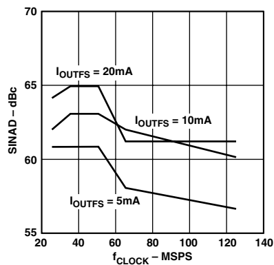
Figure 12. SINAD vs. f_{\text{CLOCK}} and I_{\text{OUTFS}} @ f_{\text{OUT}} = 5 \text{ MHz} and 0 dBFS
