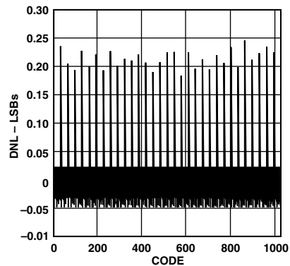
TPC 12. Typical DNL
