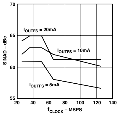
TPC 10. SINAD vs. f_{\text{CLK}} and I_{\text{OUTFS}} @ f_{\text{OUT}} = 5 \text{ MHz} and 0 \text{ dBFS}
