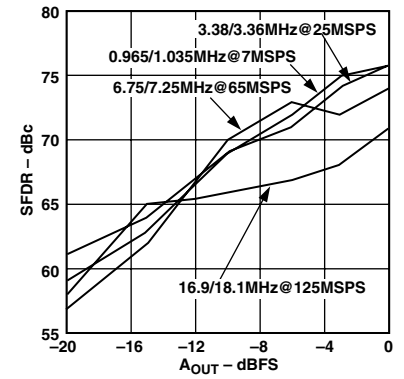
TPC 9. Dual-Tone SFDR vs. A_{OUT} @ f_{OUT} = f_{CLOCK}/7
