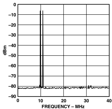
TPC 16. Dual-Tone SFDR @ f_{\text{CLK}} = 125 \text{ MSPS}
