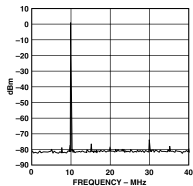
TPC 15. Single-Tone SFDR @ f_{\text{CLK}} = 125 \text{ MSPS}
