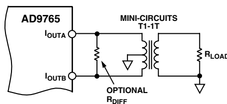
Figure 33. Differential Output Using a Transformer
