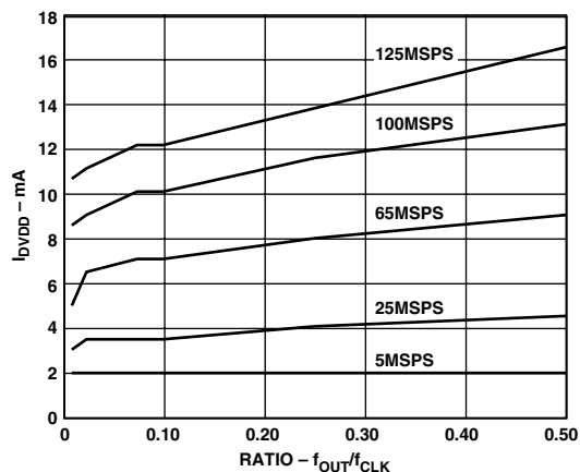
Figure 32. I_{DVDD} vs. Ratio @ DVDD = 3\text{ V}
