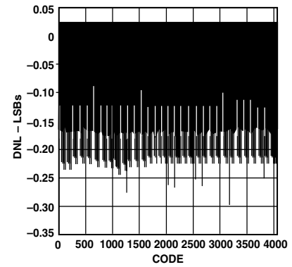
Figure 14. Typical DNL
