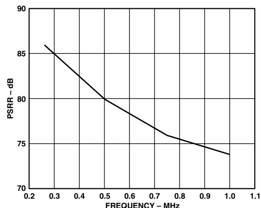
Figure 38. Power Supply Rejection Ratio of AD9767
