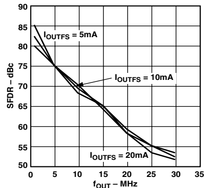
Figure 8. SFDR vs. f_{OUT} and I_{OUTFS} @ 65 MSPS and 0 dBFS
