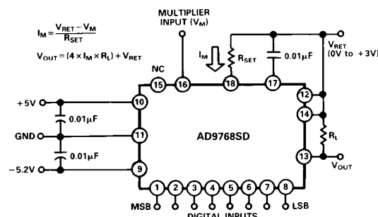
Figure 1. Conventional AD9768SD
