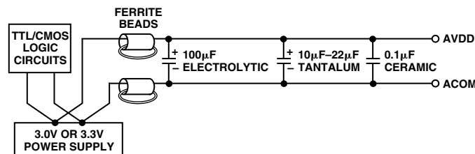
Figure 29. Differential LC Filter for 3 V or 3.3 V
