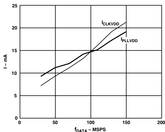
Figure 23. I_{PLLVD} and I_{CLKVD} vs. f_{DATA}
