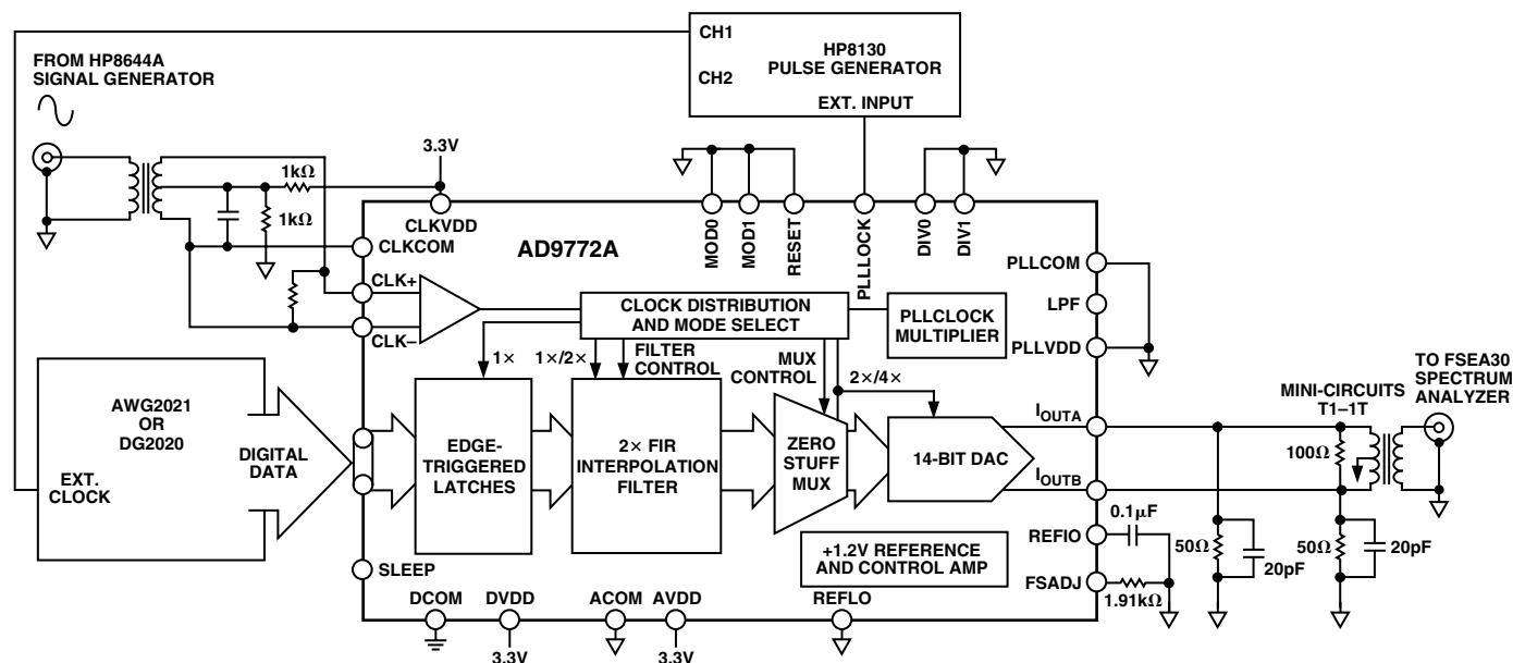
Figure 3. Basic AC Characterization Test Setup
