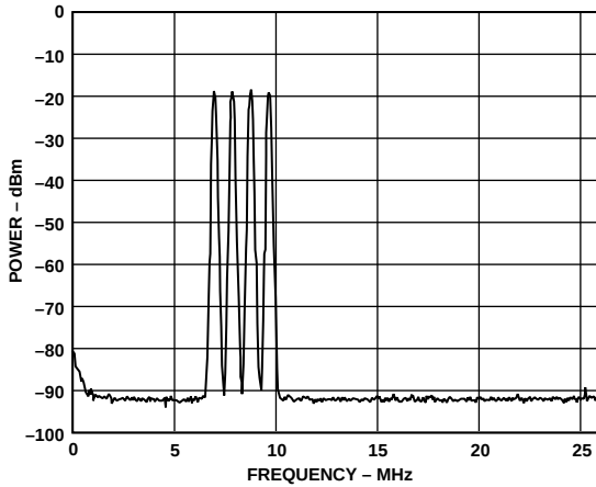
Figure 49. Spectral Plot of AD9772 Reconstructing Four GSM Modulated Carriers @ f_{DATA} = 52 MSPS, PLLVDD = 0
