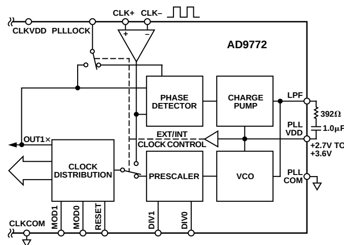
Figure 26. Clock Multiplier with PLL Clock Multiplier Enabled
