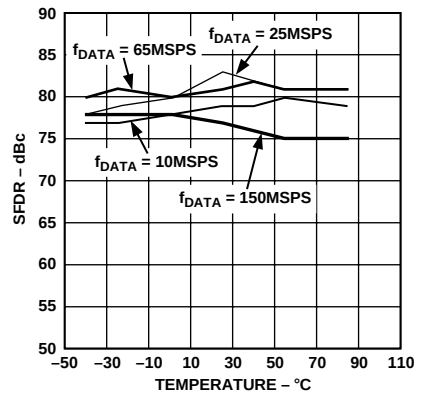
Figure 21. "In-Band" Single-Tone SFDR vs. Temperature @ f_{OUT} = f_{DATA}/11 , A_{OUT} = 0 \text{ dBFS}
