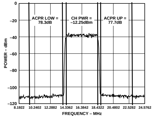
Figure 50. AD9772 Achieves 78 dB ACPR Performance Reconstructing a "WCDMA-Like" Test Vector with f_{DATA} = 65.536 MSPS and PLLVDD = 0
