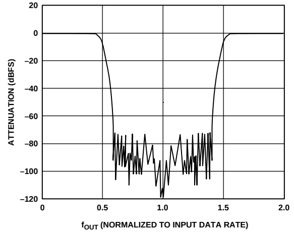
Figure 2. 2× Interpolating Filter Response
