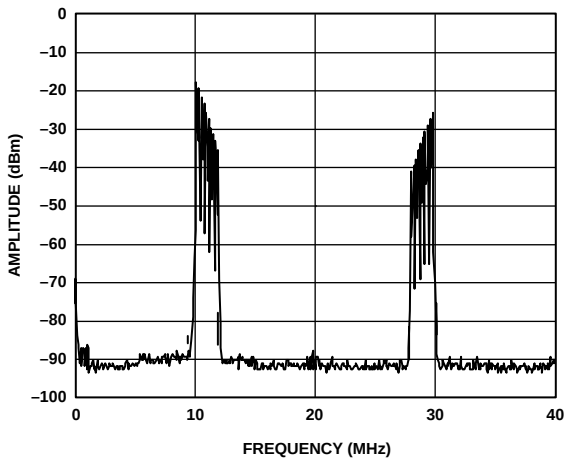
Figure 93. AD9773 Real DAC Output of Complex Input Signal Near Baseband (Negative Frequencies Only), Interpolation = 4\times , Complex Modulation in AD9773 = -f_{DAC}/4
