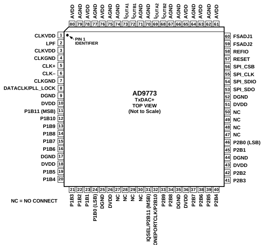
Figure 5. Pin Configuration
