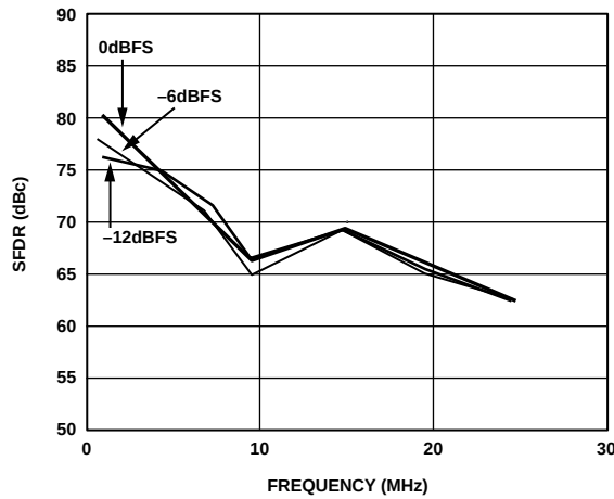
Figure 8. Out-of-Band SFDR vs. f_{\text{OUT}} @ f_{\text{DATA}} = 65\text{ MSPS}
