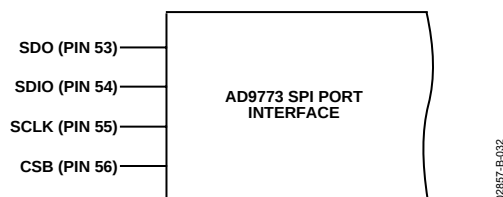
Figure 32. SPI Port Interface
