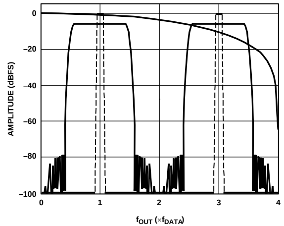
Figure 69. 4x Interpolation, Modulation = f_{DAC}/4
