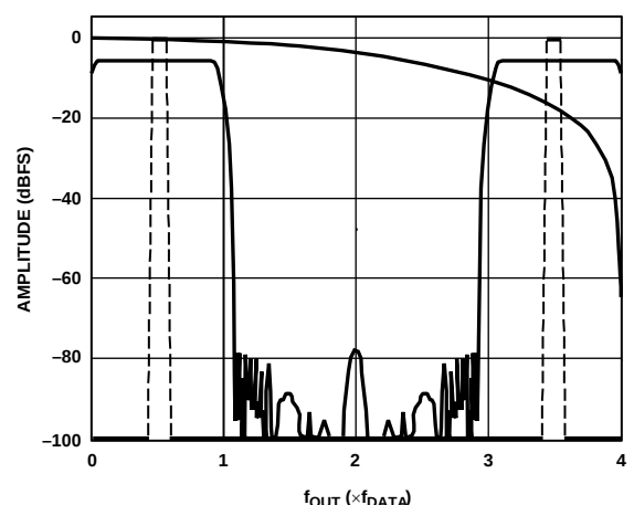
Figure 70. 4x Interpolation, Modulation = f_{DAC}/8
