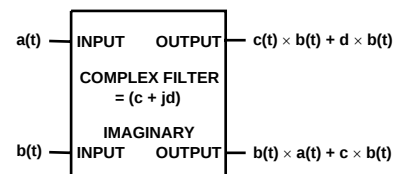
Figure 76. Realization of a Complex System
