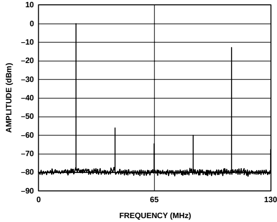
Figure 6. Single-Tone Spectrum @ f_{\text{DATA}} = 65\text{ MSPS} with f_{\text{OUT}} = f_{\text{DATA}}/3
