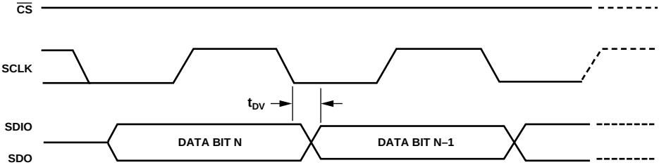
Figure 36. Timing Diagram for Register Read from AD9773
