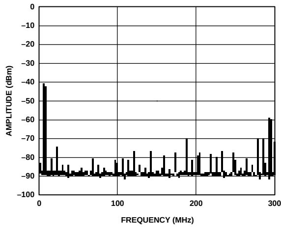
Figure 30. Single-Tone Spurious Performance, f_{OUT} = 10 MHz, f_{DATA} = 50 MSPS, Interpolation = 8×
