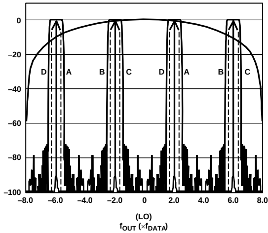
Figure 85. 8x Interpolation, Complex f_{DAC}/4 Modulation
