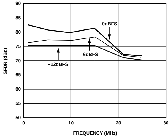
Figure 7. In-Band SFDR vs. f_{\text{OUT}} @ f_{\text{DATA}} = 65\text{ MSPS}
