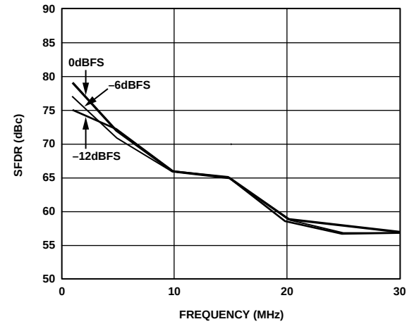
Figure 11. Out-of-Band SFDR vs. f_{\text{OUT}} @ f_{\text{DATA}} = 78\text{ MSPS}
