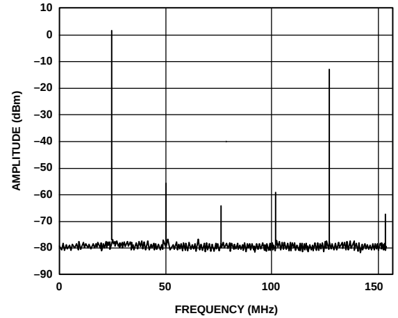
Figure 9. Single-Tone Spectrum @ f_{\text{DATA}} = 78\text{ MSPS} with f_{\text{OUT}} = f_{\text{DATA}}/3
