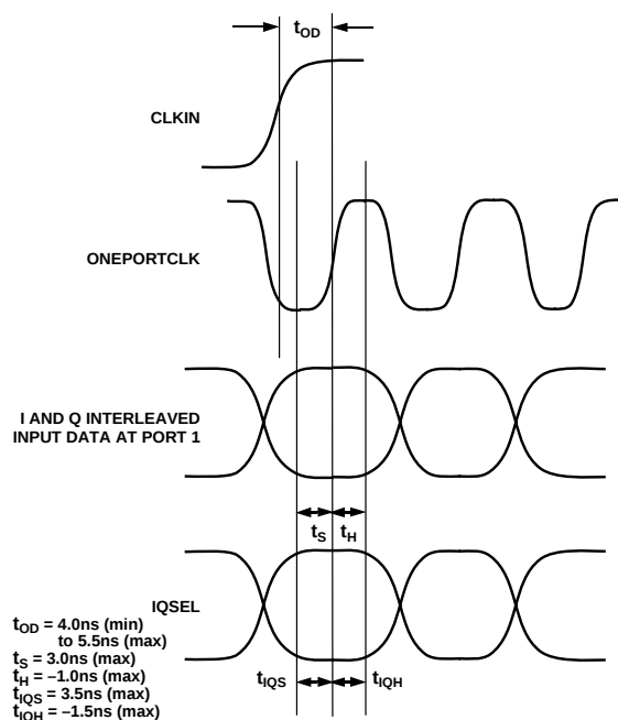
Figure 56. Timing Requirements in One-Port Input Mode with DLL Disabled
