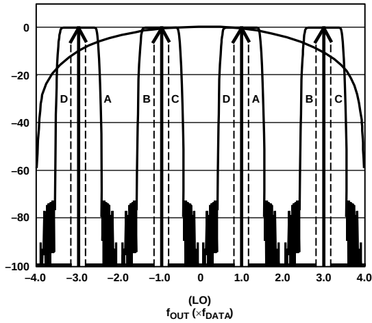
Figure 84. 4x Interpolation, Complex f_{DAC}/4 Modulation
