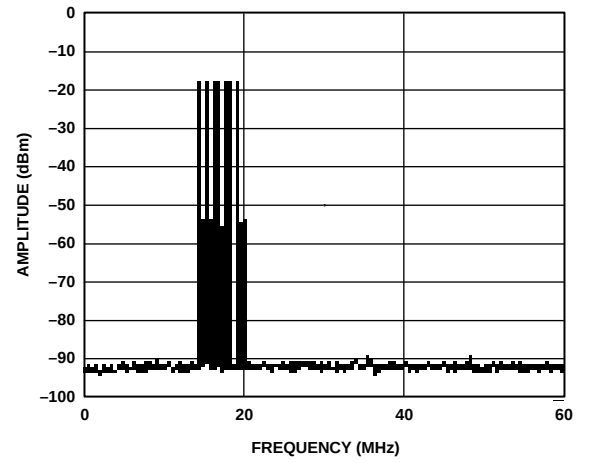
Figure 31. Eight-Tone IMD Performance, f_{DATA} = 160 MSPS, Interpolation = 8×
