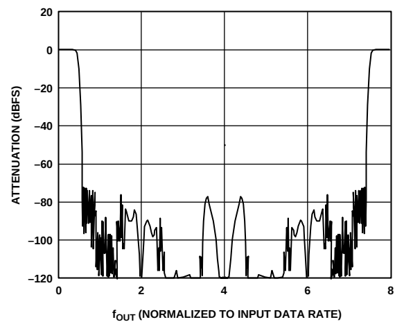
Figure 4. 8× Interpolating Filter Response
