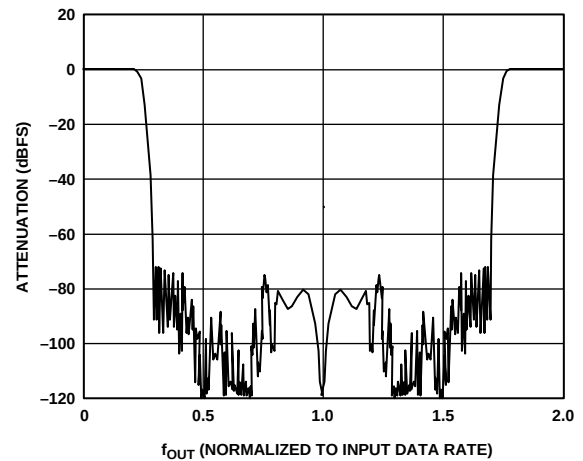
Figure 3. 4× Interpolating Filter Response
