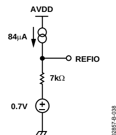
Figure 38. Internal Reference Equivalent Circuit
