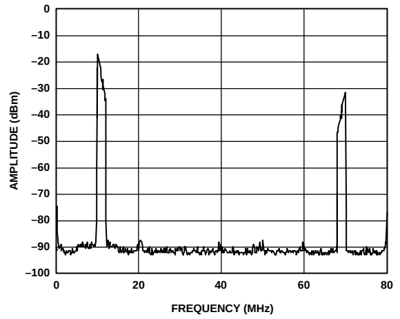
Figure 95. AD9773 Real DAC Output of Complex Input Signal Near Baseband (Positive Frequencies Only), Interpolation = 8\times , Complex Modulation in AD9773 = +f_{DAC}/8
