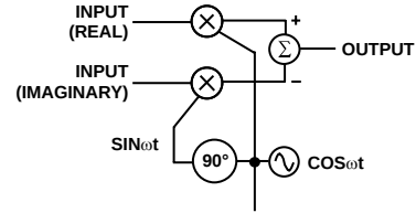
Figure 78. Quadrature Modulator
