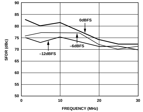
Figure 10. In-Band SFDR vs. f_{\text{OUT}} @ f_{\text{DATA}} = 78\text{ MSPS}
