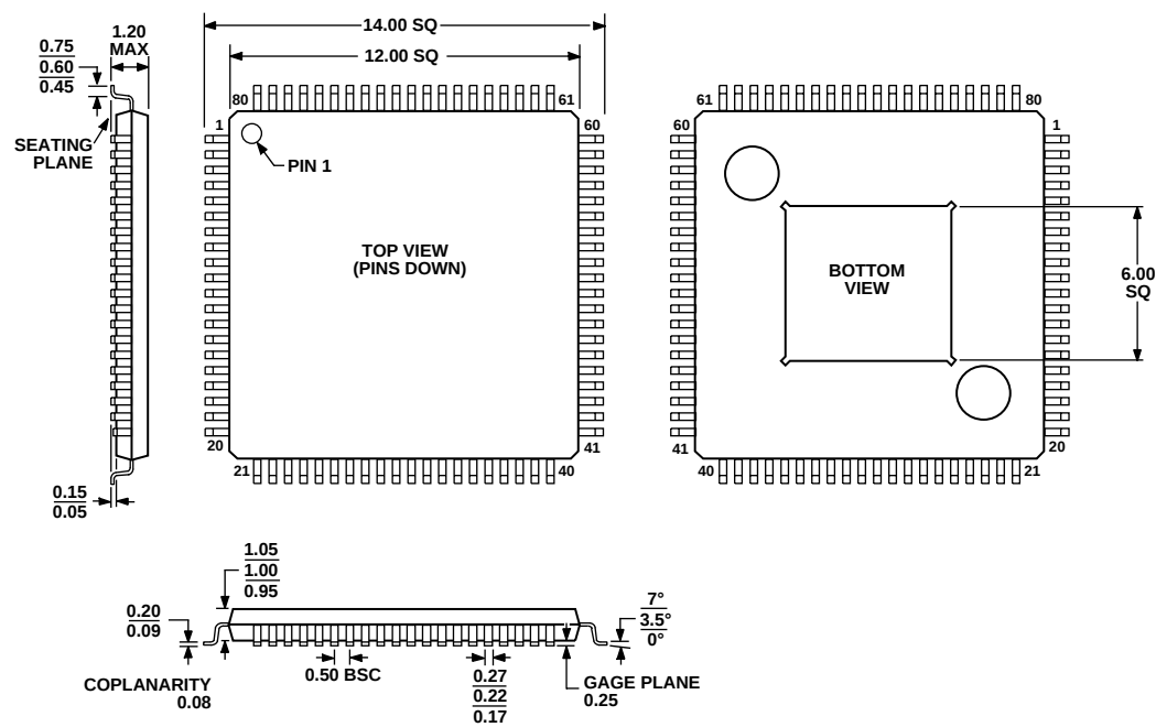
Figure 115. 80-Lead Thin Plastic Quad Flat Package, Exposed Pad [TQFP/ED] (SV-80)
