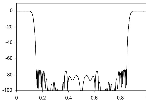
Figure 1b. 4x Interpolating Filter Response
