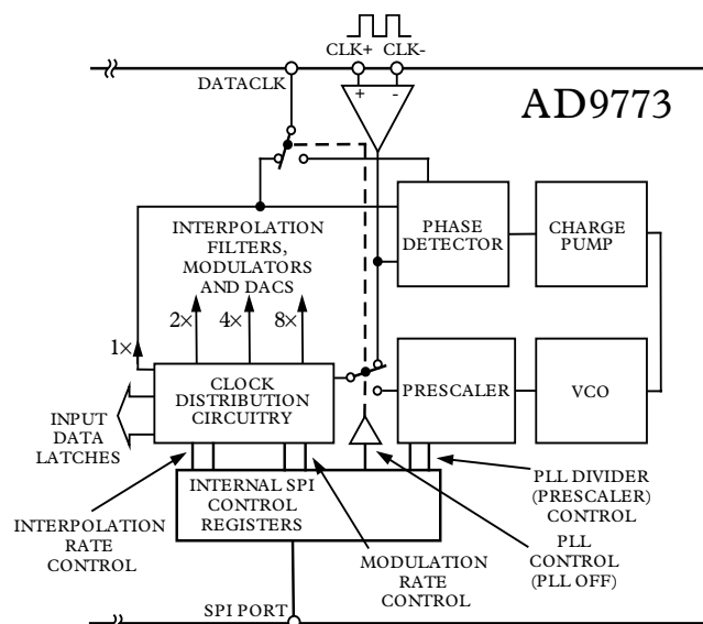
Figure 8. AD9773 PLL and Clock Circuitry with PLL Disabled
