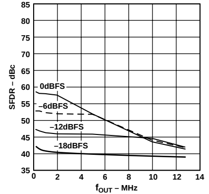
Figure 6. "Out-of-Band" SFDR vs. f_{OUT} @ 32 MSPS ( \text{CLKIN}/2 to 3 \frac{1}{2} \text{CLKIN} )
