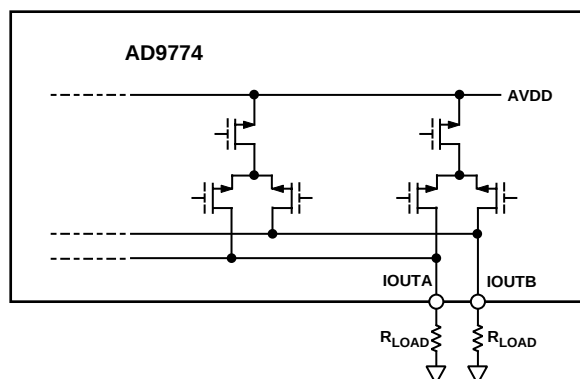
Figure 31. Equivalent Analog Output Circuit
