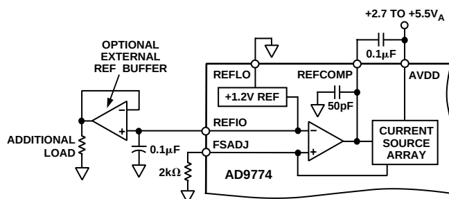
Figure 27. Internal Reference Configuration
