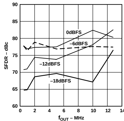
Figure 5. "Inband" SFDR vs. f_{OUT} @ 32 MSPS (DC to \text{CLKIN}/2 )
