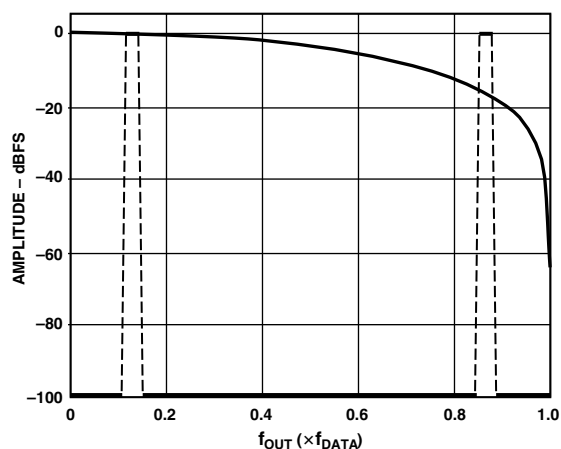
Figure 26d. No Interpolation, Modulation = f_{DAC}/8
