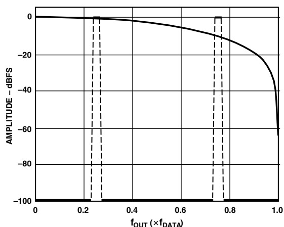
Figure 26c. No Interpolation, Modulation = f_{DAC}/4
