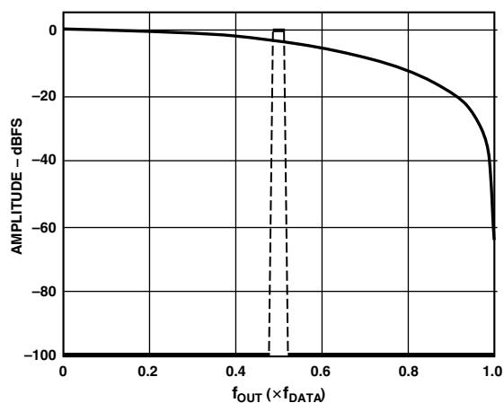
Figure 26b. No Interpolation, Modulation = f_{DAC}/2
