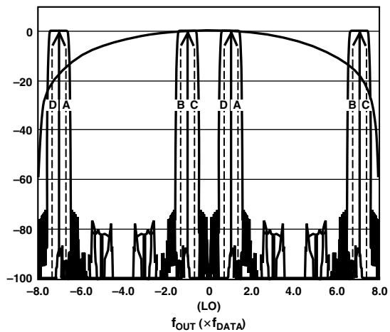
Figure 43. 8x Interpolation, Complex f_{DAC}/8 Modulation
