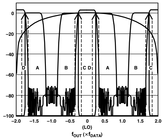
Figure 41. 2x Interpolation, Complex f_{DAC}/8 Modulation
