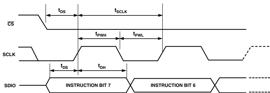
Figure 4. Timing Diagram for Register Write to AD9775
