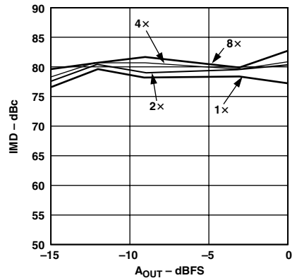
TPC 14. Third Order IMD Products vs. A_{OUT} and Interpolation Rate f_{DATA} = 50 MSPS for All Cases, 1x f_{DAC} = 50 MSPS 2x f_{DAC} = 100 MSPS 4x f_{DAC} = 200 MSPS 8x f_{DAC} = 400 MSPS
