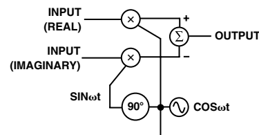
Figure 33. Quadrature Modulator
