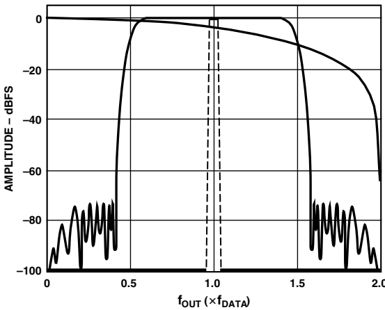
Figure 27b. 2× Interpolation, Modulation = f_{DAC}/2
