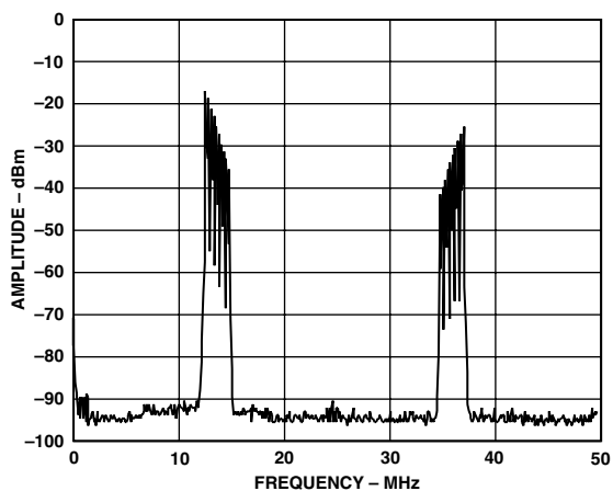
Figure 48. AD9775, Real DAC Output of Complex Input Signal Near Baseband (Negative Frequencies Only), Interpolation = 4x, Complex Modulation in AD9775 = -f_{DAC}/4
