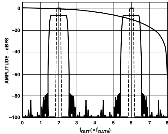
Figure 29c. 8× Interpolation, Modulation = f_{DAC}/4
