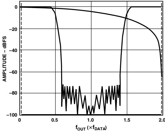
Figure 27a. 2× Interpolation, Modulation = Disabled
