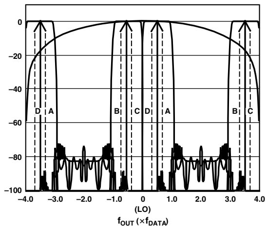
Figure 42. 4x Interpolation, Complex f_{DAC}/8 Modulation
