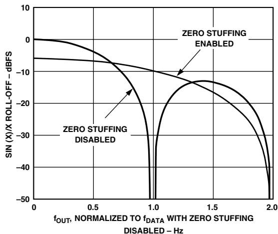
Figure 30. Effect of Zero Stuffing on DAC's SIN(x)/x Response
