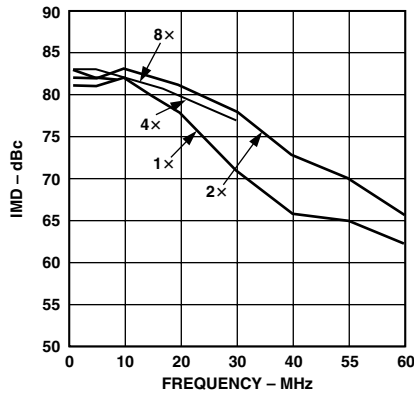
TPC 13. Third Order IMD Products vs. f_{OUT} and Interpolation Rate, 1x f_{DATA} = 160 MSPS 2x f_{DATA} = 160 MSPS 4x f_{DATA} = 80 MSPS 8x f_{DATA} = 50 MSPS
