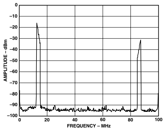
Figure 50. AD9775, Real DAC Output of Complex Input Signal Near Baseband (Positive Frequencies Only), Interpolation = 8x, Complex Modulation in AD9775 = +f_{DAC}/8
