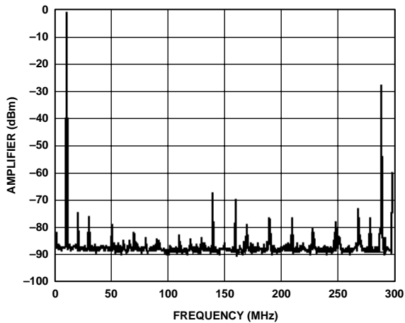
Figure 26. Single-Tone Spurious Performance, f_{OUT} = 10 MHz, f_{DATA} = 150 MSPS, Interpolation = 2x
