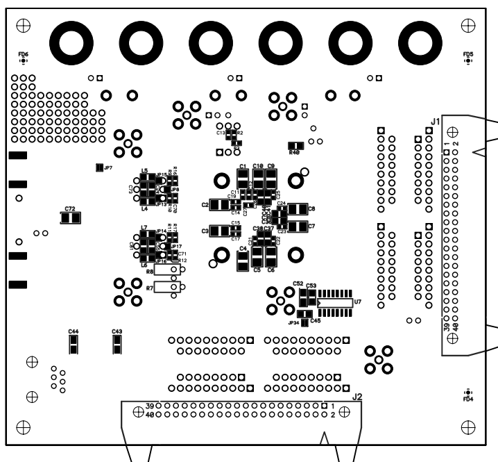
Figure 63. AD9775 Evaluation Board Components, Top Side
