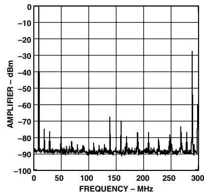
TPC 21. Single-Tone Spurious Performance, f_{OUT} = 10\text{ MHz} , f_{DATA} = 150\text{ MSPS} , Interpolation = 2\times
