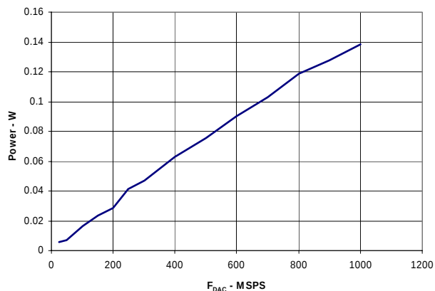
Figure 23. Power Dissipation of Inverse Sinc Filter
