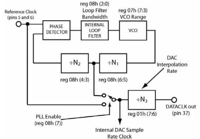
Figure 32. Internal Clock Architecture of AD9776
