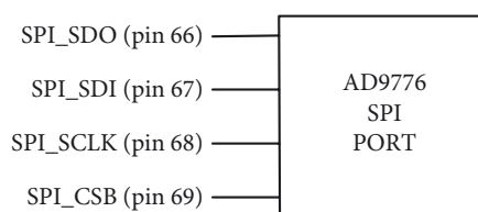
Figure 24. AD9776 SPI Port
