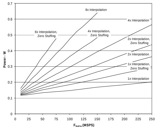
Figure 21. Power Dissipation, Single DAC Mode
