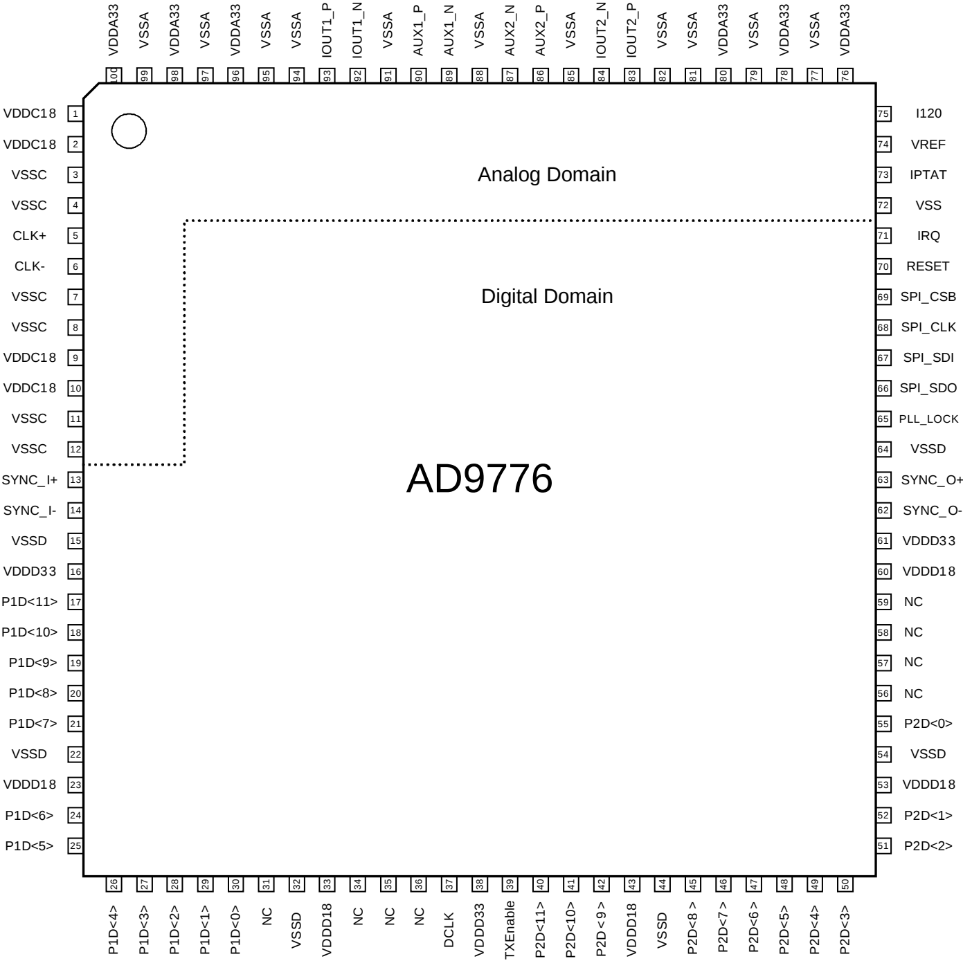
Figure 2. Pin Configuration
