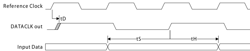
Figure 34. Timing Specifications for AD9776, PLL Enabled, Reference Clock = 2x Input Sample Rate
