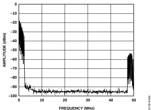
Figure 89. AD9777, Real DAC Output of Complex Input Signal Near Baseband (Positive Frequencies Only), Interpolation = 4x, No Modulation in AD9777
