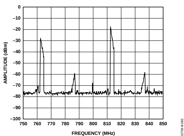
Figure 92. AD9777 Complex Output from Figure 91, Now Quadrature Modulated by AD8345 (LO = 800 MHz)
