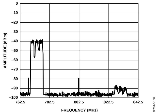
Figure 100. AD9777/AD8345 Synthesizing a Three-Carrier WCDMA Signal at an LO of 800 MHz
