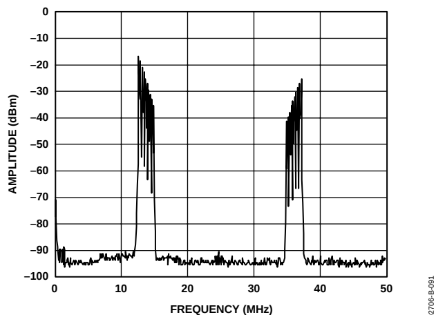
Figure 91. AD9777, Real DAC Output of Complex Input Signal Near Baseband (Positive Frequencies Only), Interpolation = 4x, Complex Modulation in AD9777 = +f_{DAC}/4
