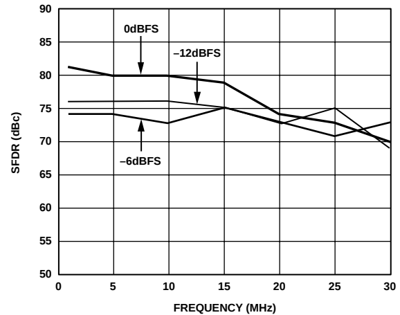
Figure 11. Out-of-Band SFDR vs. f_{\text{OUT}} @ f_{\text{DATA}} = 78\text{ MSPS}
