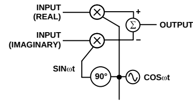
Figure 78. Quadrature Modulation
