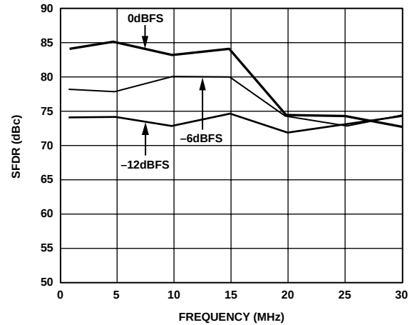
Figure 10. In-Band SFDR vs. f_{\text{OUT}} @ f_{\text{DATA}} = 78\text{ MSPS}
