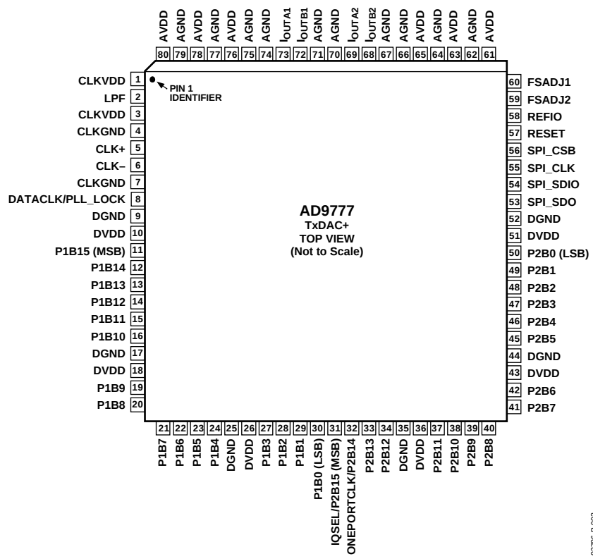
Figure 5. Pin Configuration
