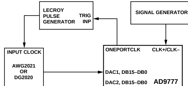
JUMPER CONFIGURATION FOR ONE PORT MODE PLL OFF
