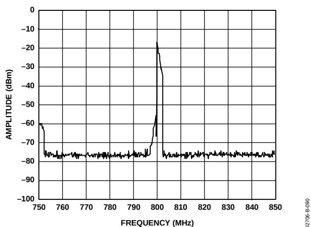
Figure 90. AD9777 Complex Output from Figure 89, Now Quadrature Modulated by AD8345 (LO = 800 MHz)
