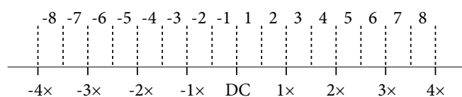
Figure 39. Nyquist Zones
