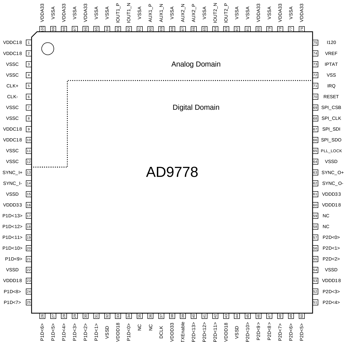
Figure 2. Pin Configuration
