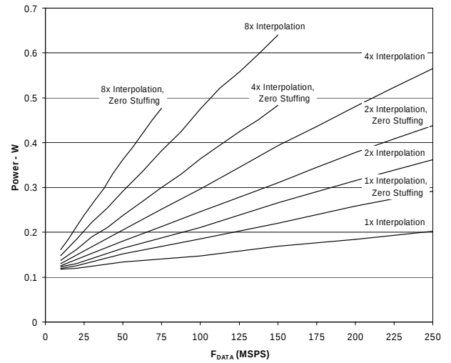
Figure 21. Power Dissipation, Single DAC Mode
