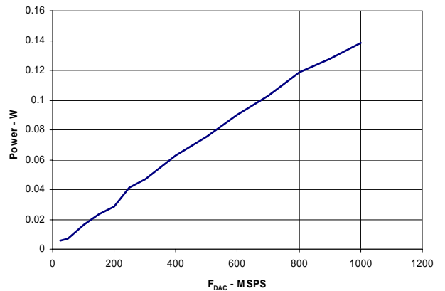
Figure 23. Power Dissipation of Inverse Sinc Filter
