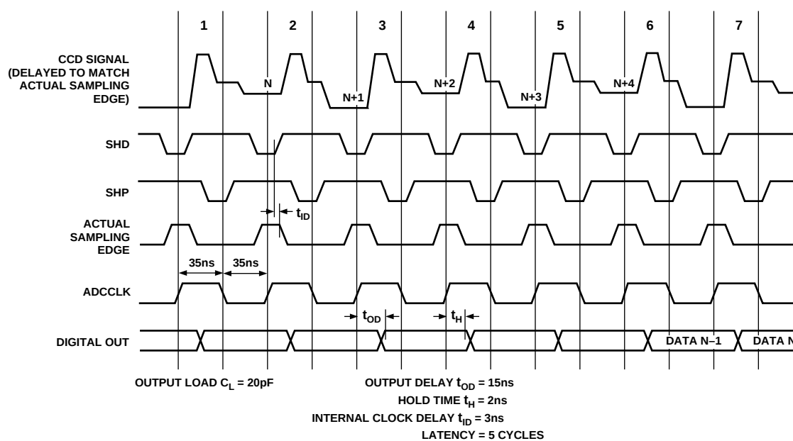
Figure 12. Timing Diagram
