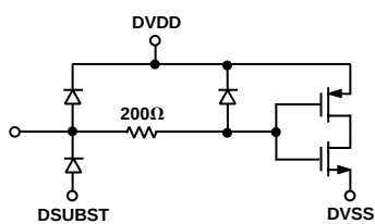
Figure 3. Pin 16 (ADCCLK)
