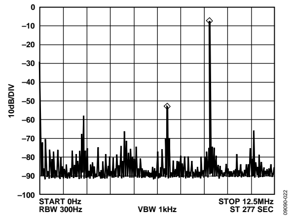
Figure 22. f_{CLK} = 25 \text{ MHz} , f_{OUT} = 9.1 \text{ MHz} , Frequency Word = 0x5D2F1AA0
