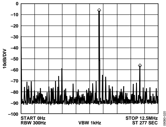
Figure 20. f_{CLK} = 25 \text{ MHz} , f_{OUT} = 7.1 \text{ MHz} , Frequency Word = 0x48B43958
