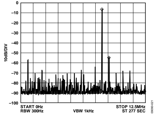
Figure 21. f_{CLK} = 25 \text{ MHz} , f_{OUT} = 8.1 \text{ MHz} , Frequency Word = 0x52F1A9FC
