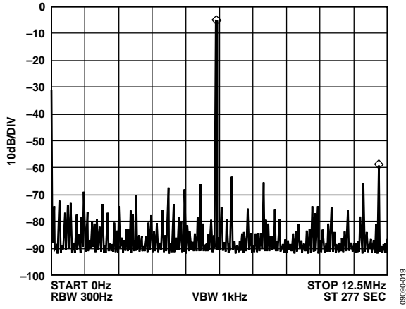
Figure 19. f_{CLK} = 25 \text{ MHz} , f_{OUT} = 6.1 \text{ MHz} , Frequency Word = 0x3E76C8B4
