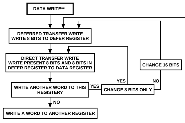
Figure 24. Data Writes
