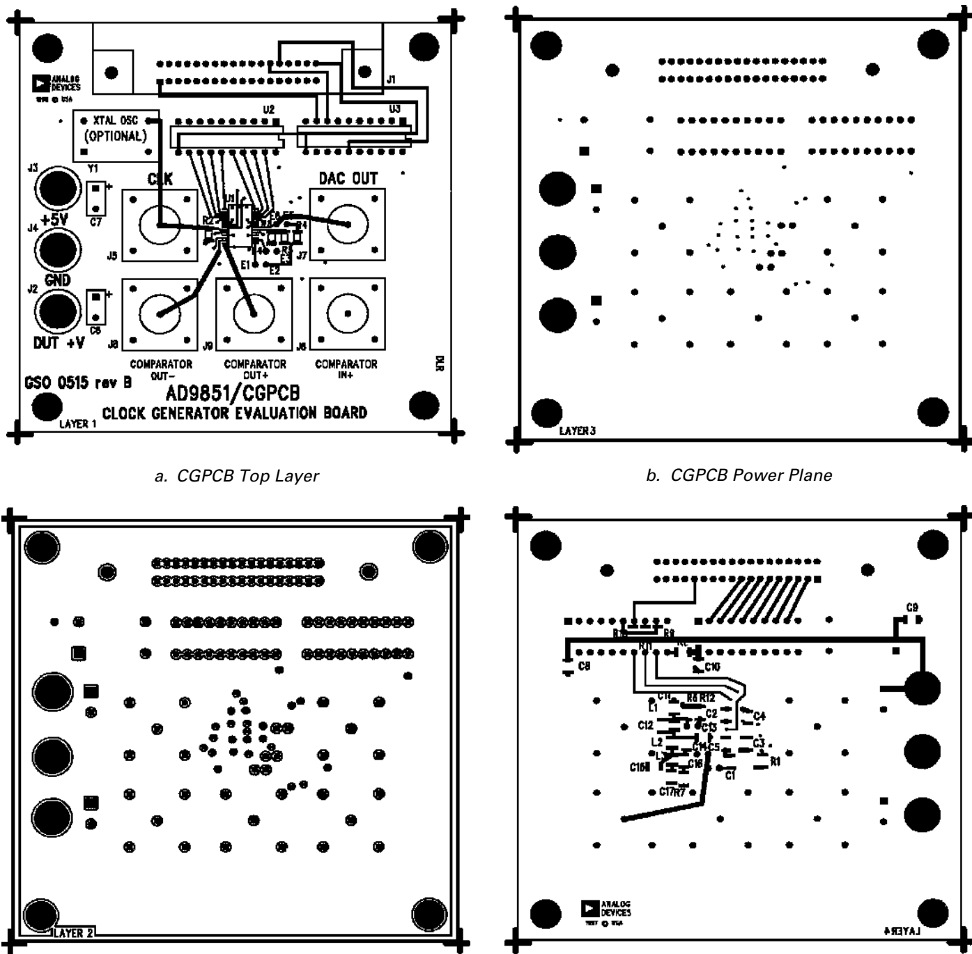
c. CGPCB Ground Plane
