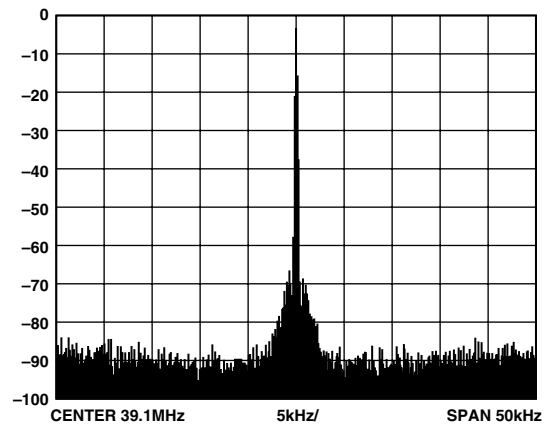
TPC 12. Narrowband SFDR, 39.1 MHz, 50 kHz BW, 10 MHz REFCLK with REFCLK Multiplier = 10×
