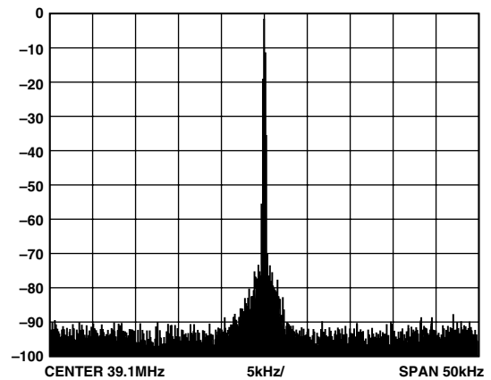
TPC 11. Narrowband SFDR, 39.1 MHz, 50 kHz BW, 30 MHz REFCLK with REFCLK Multiplier = 10×
