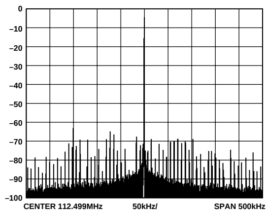
Figure 14. The Opposite of a “Sweet Spot.” 112.499 MHz with multiple high energy spurs close around the fundamental.
