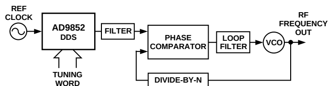
Figure 28. Agile High-Frequency Synthesizer
