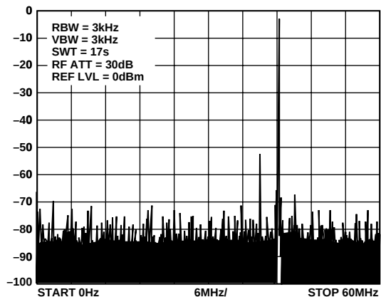
Figure 9. A_{OUT} = 42 MHz
