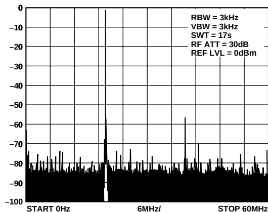
Figure 11. A_{OUT} = 20 MHz
