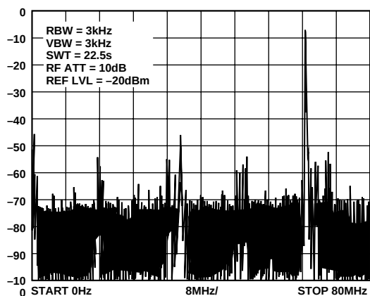
Figure 7. QPSK, 1.375 Mb/s, A_{OUT} = 65 MHz
