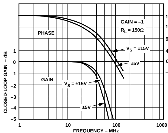
Figure 6. Closed-Loop Gain and Phase vs. Frequency, G = -1 , R_L = 150\ \Omega , R_F = 680\ \Omega for \pm 15\text{ V} , 620\ \Omega for \pm 5\text{ V}
