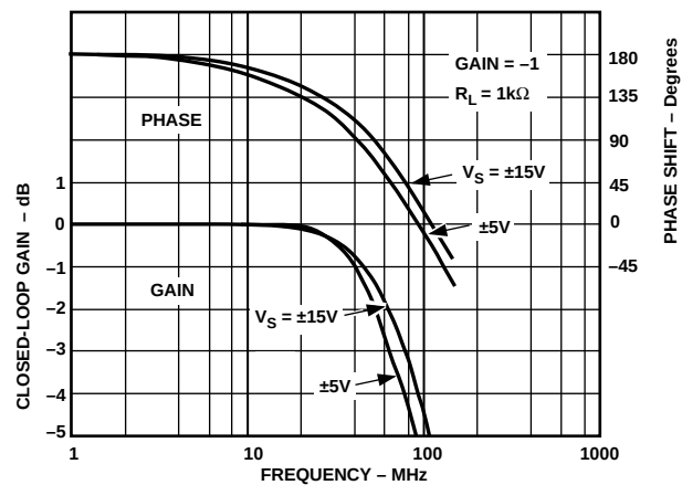
Figure 7. Closed-Loop Gain and Phase vs. Frequency, G = -1 , R_L = 1\text{ k}\Omega , R_F = 680\ \Omega for V_S = \pm 15\text{ V} , 620\ \Omega for \pm 5\text{ V}
