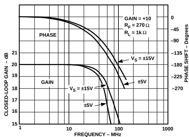
Figure 15. Closed-Loop Gain and Phase vs. Frequency, G = +10 , R_L = 1 \text{ k}\Omega
