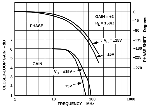
Figure 10. Closed-Loop Gain and Phase vs. Frequency, G = +2 , R_L = 150\Omega , R_F = 750\Omega for \pm 15V , 715\Omega for \pm 5V
