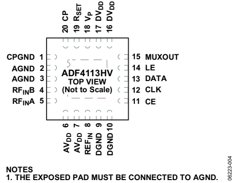
Figure 4. LFCSP Pin Configuration
