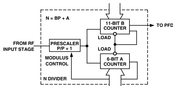
Figure 4. A and B Counters
