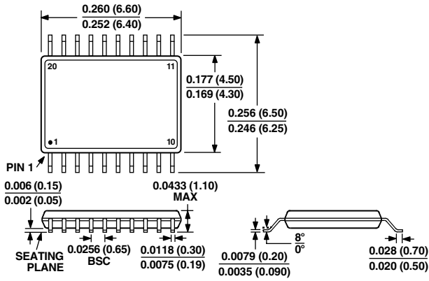
Thin Shrink Small Outline Package (TSSOP) (RU-20)
