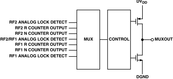
Figure 6. MUXOUT Circuit
