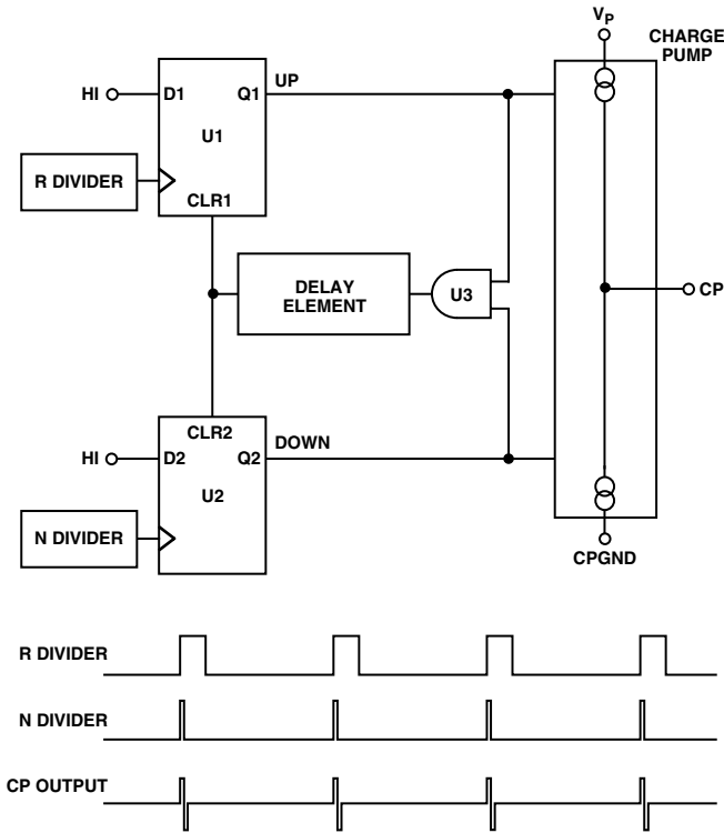
Figure 5. PFD Simplified Schematic and Timing (In Lock)
