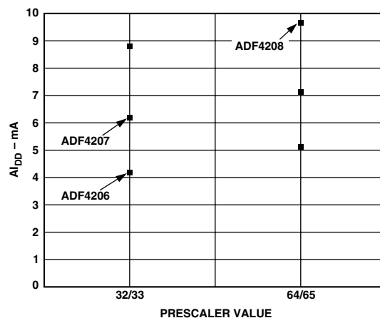
TPC 17. ADF4206/ADF4207/ADF4208 I_{DD} vs. Prescaler Value (RF1)
