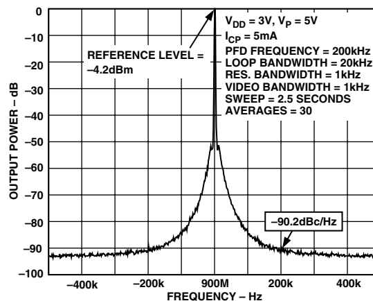
TPC 4. ADF4208 RF1 Reference Spurs (900 MHz, 200 kHz, 20 kHz)
