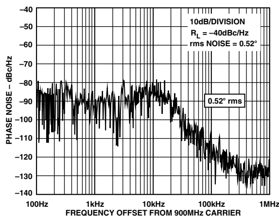
TPC 5. ADF4208 RF1 Integrated Phase Noise (900 MHz, 200 kHz, 20 kHz)
