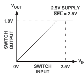
Figure 8. 2.5 V to 1.8 V Voltage Translation, \overline{SEL} = 2.5 V
