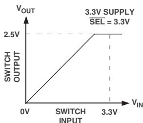
Figure 6. 3.3 V to 2.5 V Voltage Translation, \overline{SEL} = 3.3 V
