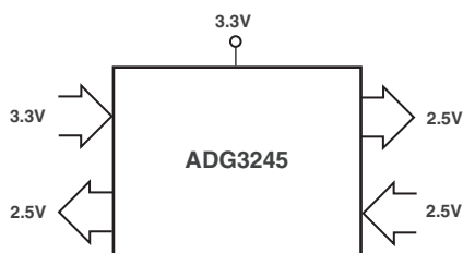
Figure 5. 3.3 V to 2.5 V Voltage Translation, \overline{SEL} = 3.3 V
