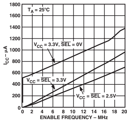
TPC 9. I_{CC} vs. Enable Frequency
