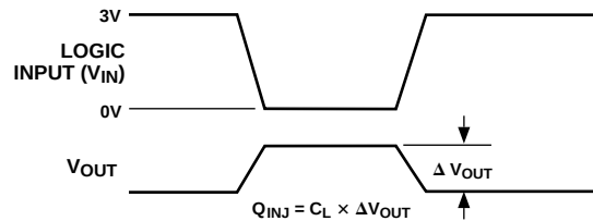
Test Circuit 10. Charge Injection
