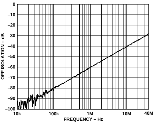
Figure 15. Off Isolation of the ADG466, V_{DD}/V_{SS} = 0 V and Input Signal Level of \pm 100 mV
