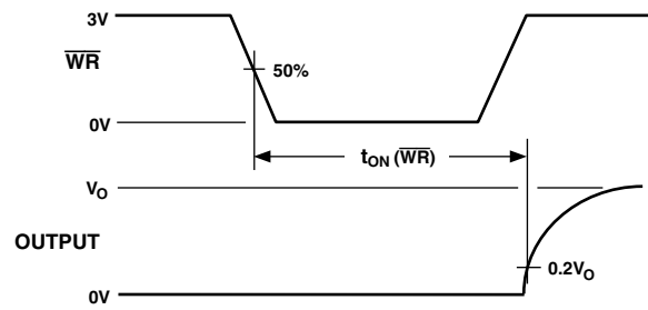
Test Circuit 10. Write Turn-On Time, t_{ON} (\overline{WR})
