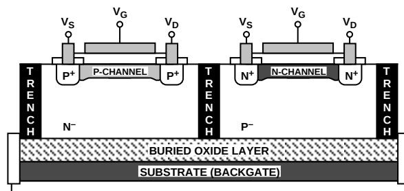
Figure 10. Trench Isolation
