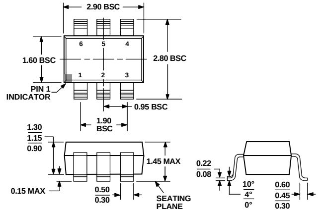
Figure 22. 6-Lead Small Outline Transistor Package [SOT-23] (RT-6) Dimensions shown in millimeters
