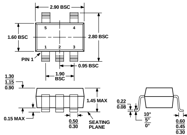
Figure 23. 5-Lead Small Outline Transistor Package [SOT-23] (RJ-5) Dimensions shown in millimeters
