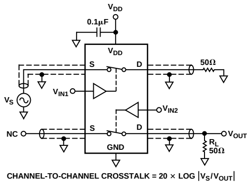
Test Circuit 8. Channel-to-Channel Crosstalk
