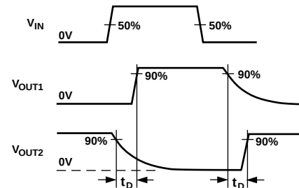
Test Circuit 5. Break-Before-Make Time Delay, t_D
