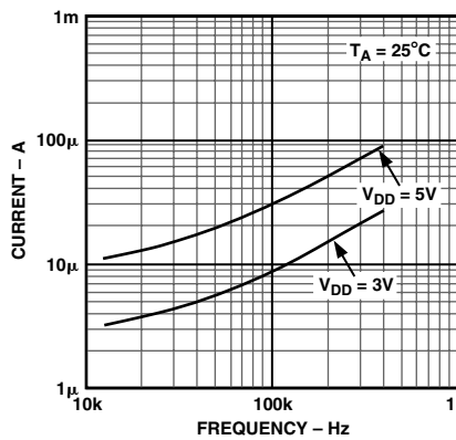
Figure 9. Input Current vs. Switching Frequency
