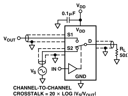
Test Circuit 7. Channel-to-Channel Crosstalk \text{CROSSTALK} = 20 \times \log |V_S/V_{OUT}|
