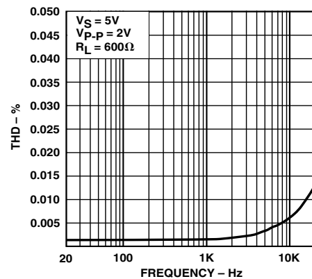
TPC 12. THD
